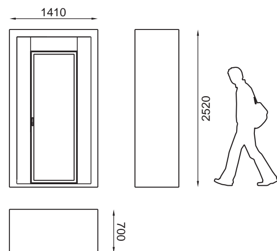
BALCONYDOOR TOTEM boiserie ST-PB/PB-01/CV-PB-01
