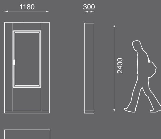
WINDOW CONCEPT S white SB-F/F-05/CV-F-05
