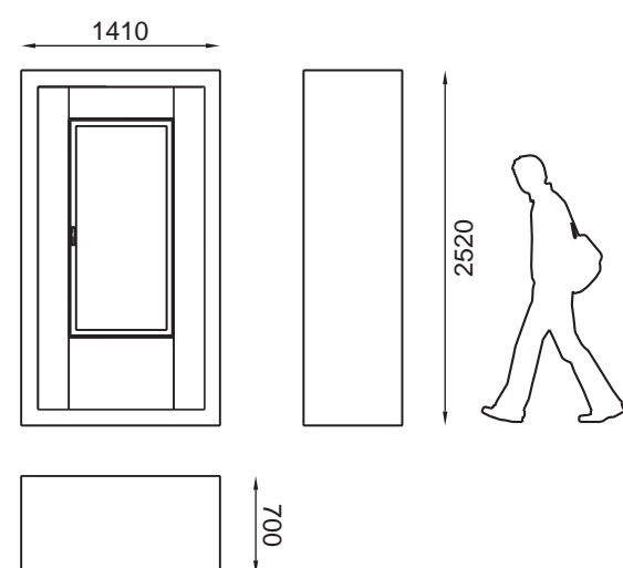
WINDOW TOTEM boiserie ST-F/F-01/CV-F-01
