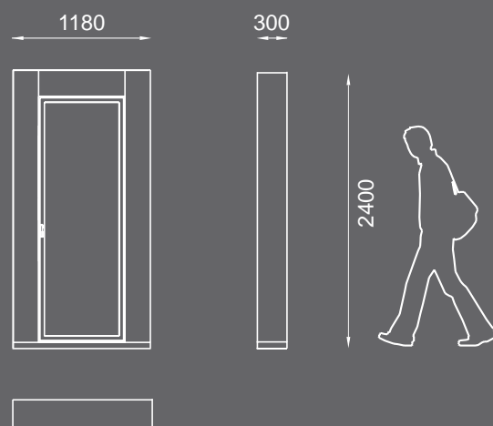
BALCONYDOOR CONCEPT S white SB-PB/PB-05/CV-PB-05
