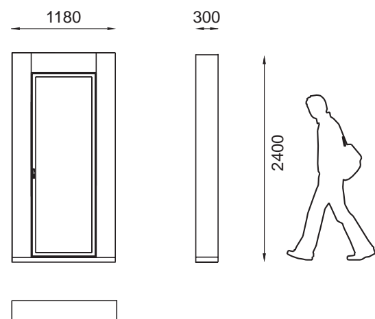
BALCONYDOOR CONCEPT S boiserie SB-PB/PB-01/CV-PB-01
