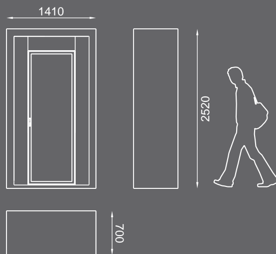
BALCONYDOOR TOTEM white ST-PB/PB-05/CV-PB-05
